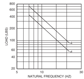
Load vs. Natural Frequency
