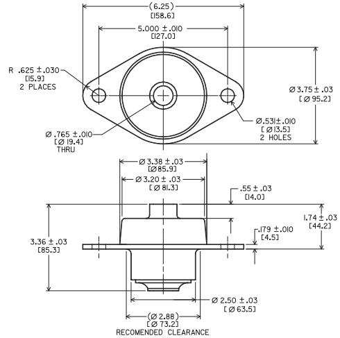
AXIAL STATIC LOAD RANGE - 562SL
