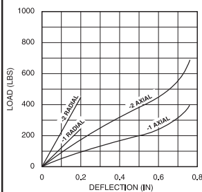
Load vs. Deflection
