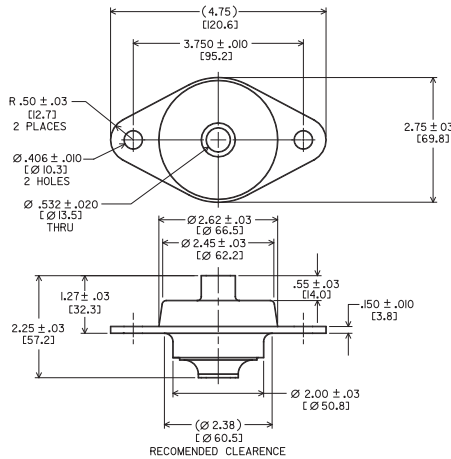
AXIAL STATIC LOAD RANGE - 558SL
